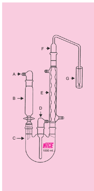
8098 - Monier Williams Apparatus (Sulphur dioxide assembly), NICE®
