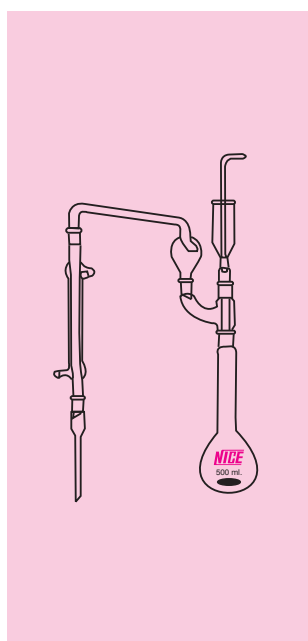
8101 - Kjeldahl Distillation Assembly, NICE®
